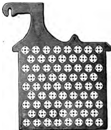
FIG. 313.—One Plate, or "Grid," of a Type of Storage Cell constructed by inserting buttons or ribbons of the proper chemical substances in perforations. Some such cells use crimped ribbons of metallic lead for inserting in the perforations, others pure red lead or other suitable material.
